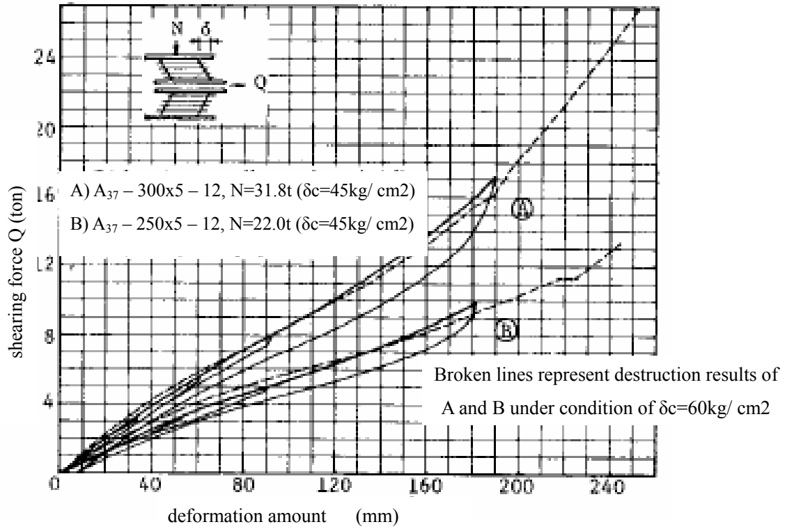
Fig.4 Compressive shearing experiment using a large-scale testing machine
