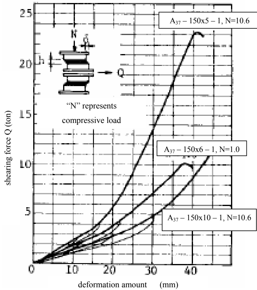
Fig. 3 destruction experiment on single-layer aseismic isolator
