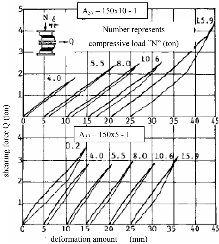
Fig.2 Compressive shearing experiment on single-layer aseismic isolators
