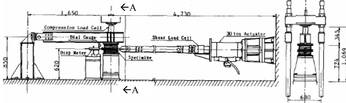
Fig.1 Two-way loading test machine
