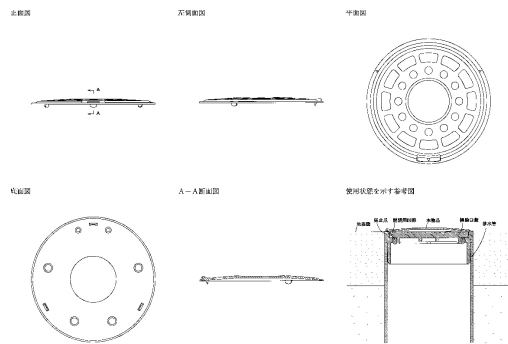
1227057AA 排水枡用掃除口蓋の養生用被覆蓋
